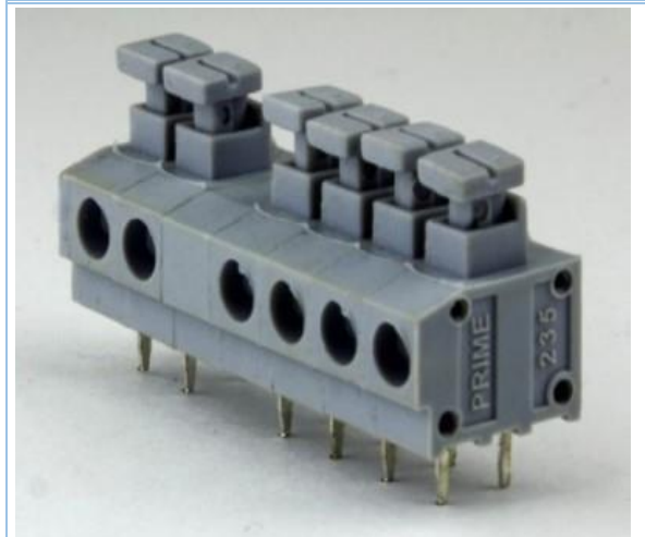
Prime PFT 235 Series
