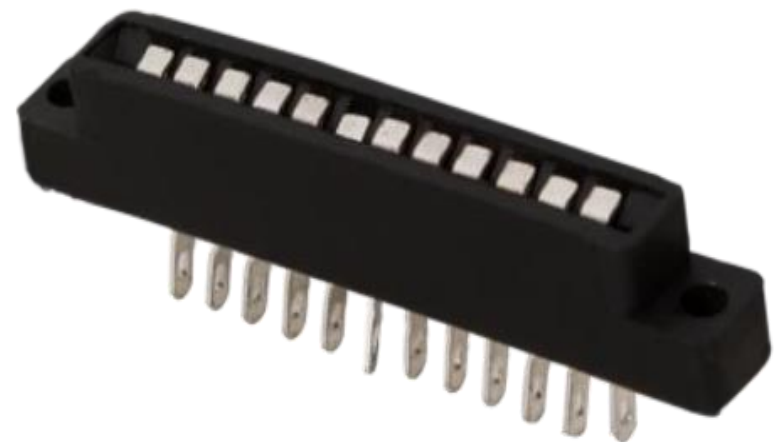
Prime PC2B Card Edge Connector
