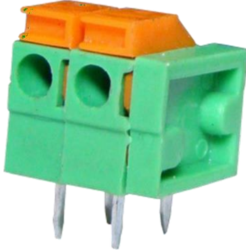
Vital PFT-H-5.00 Series
